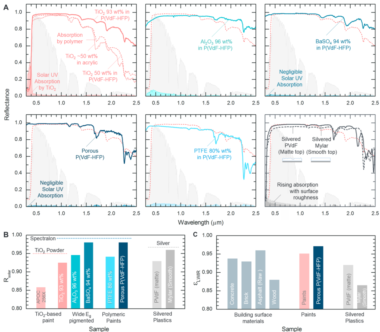
Figure 2. (A) (From top-left to bottom right) Measured spectral reflectances of paints based on \text{TiO}_2 , \text{Al}_2\text{O}_3 , \text{BaSO}_4 , porous P(VdF-HFP) and PTFE, and silvered plastics. The paint films are all \sim 1\text{mm} thick. (B) R_{\text{solar}} of paints and silvered plastics. APOC 256X paint is rated by the Cool Roof Rating Council as the most reflective on the market. The dotted lines show the reflectances of \text{TiO}_2 powder, spectralon (porous PTFE), and silver, and represent the likely upper limits of R_{\text{solar}} of \text{TiO}_2 -based, polymer-based, and silvered radiative coolers respectively. Note that the reflectances were weighted using ASTM G-173 solar spectrum, which assumes a solar zenith angle of 48.19^\circ . During summertime or in the tropics, the noon-time zenith angle is smaller. Consequently, UV light is stronger and further lowers R_{\text{solar}} of \text{TiO}_2 and silver-based designs. (C) \epsilon_{\text{LWIR}} of common building materials, paints and silvered emitters.
