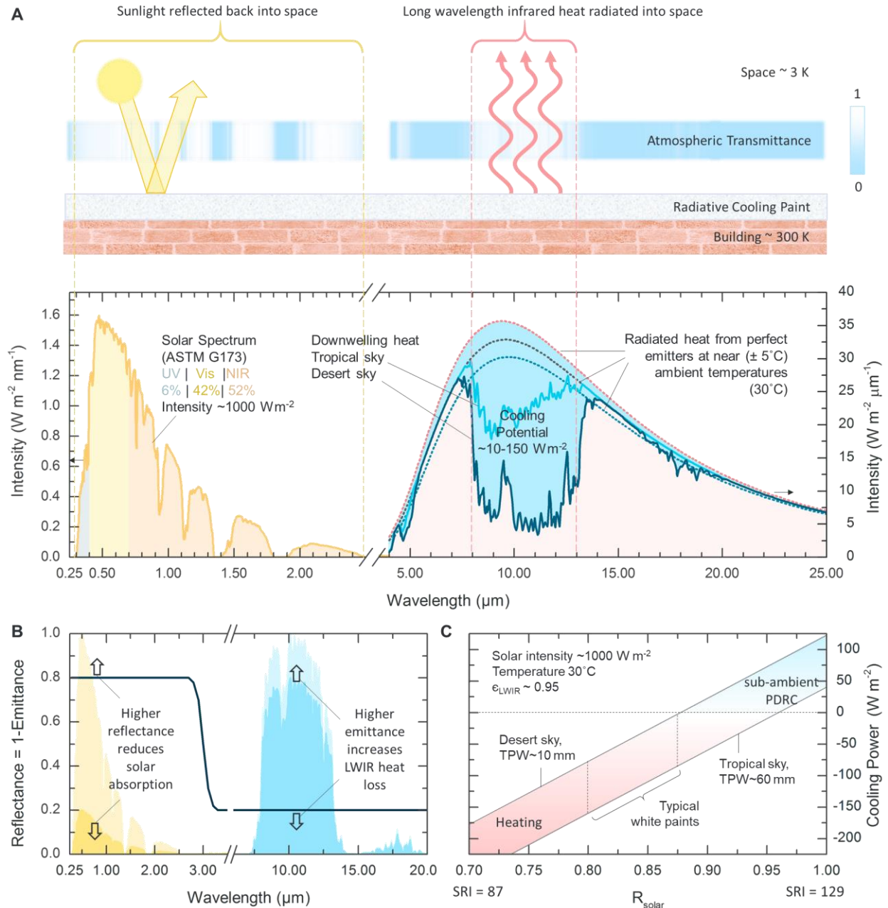
Figure 1. (A) Schematic showing passive daytime radiative cooling by solar reflection and LWIR thermal emission through the atmospheric transmission windows. Corresponding solar and thermal spectra are shown below. (B) Schematic showing how high solar reflectance and thermal emittance enable PDRC. It should be noted that at near-ambient temperatures, radiative transfer (= radiated heat from emitter – downwelling heat from sky) is small outside the LWIR window, making broadband and selective LWIR emitters similarly effective at cooling. (C) Schematic showing cooling powers (thermal emission – solar absorption) 1 of emissive coatings ( \epsilon_{\text{LWIR}} \sim 0.95 ) as a function of R_{\text{solar}} (or solar reflectance index (SRI), which varies linearly with R_{\text{solar}} ). R_{\text{solar}} > 0.95 usually yields sub-ambient radiative cooling.
